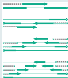
Rod or cord operation, electric drive, 2 parts, symmetric order
