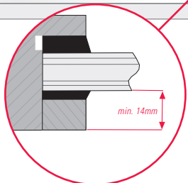
detail: rightangled window rabbet detail: sloping window rabbet
