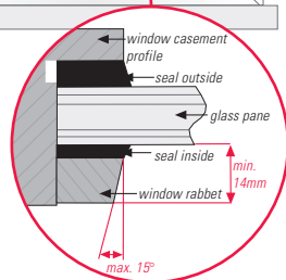
detail: rightangled window rabbet detail: sloping window rabbet
